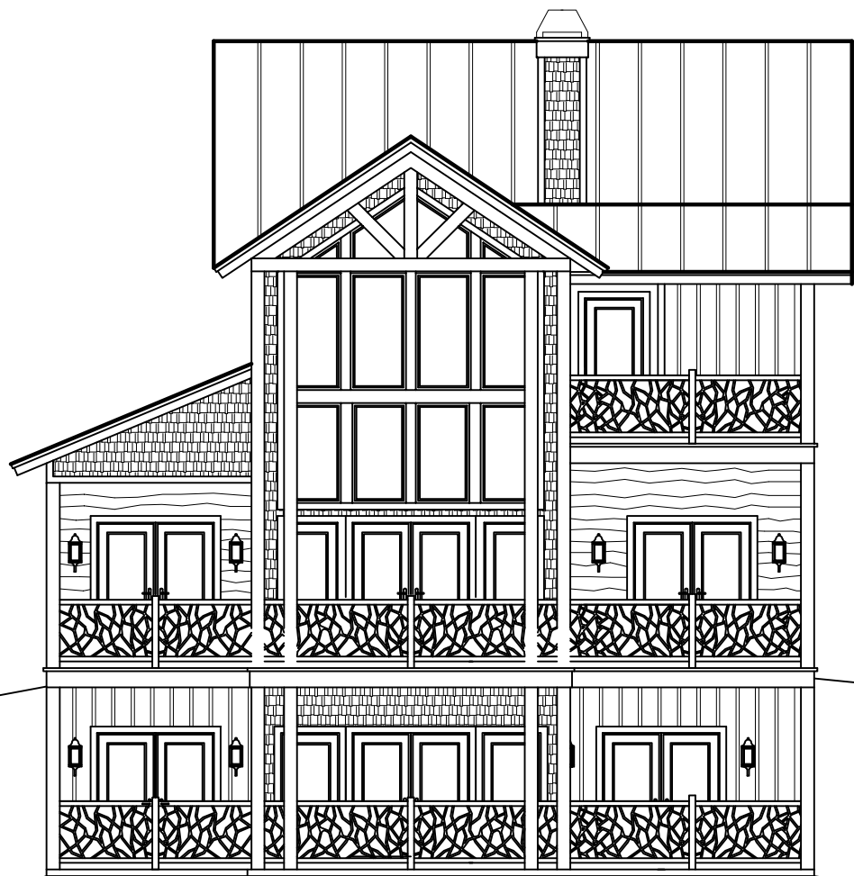
REAR ELEVATION
